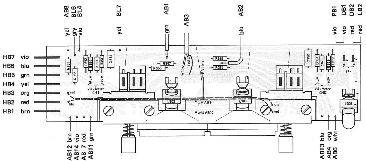
VU-Meter Board 1.077.468
